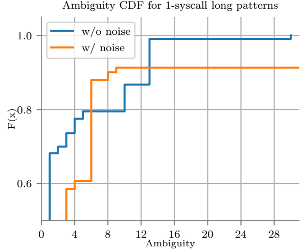
Figure 4: Total Pattern Ambiguity Comparison (1-syscall long patterns)
