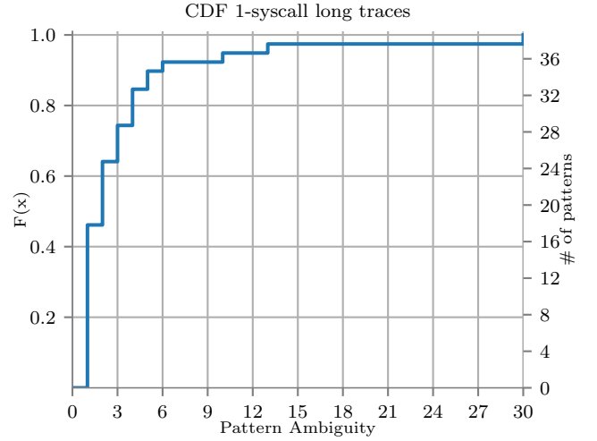
Figure 2: Pattern Ambiguity for 1-syscall long patterns
